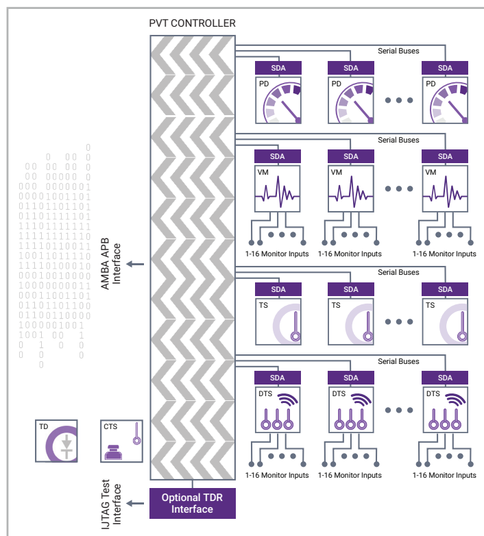
Figure 1: PVT Controller with SLM PVT Monitor IP
