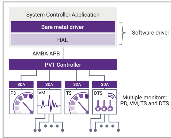
Figure 2: Reference bare metal software driver
